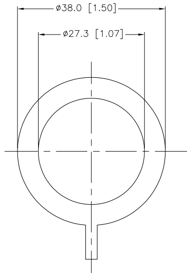
WASHER (ENCLOSED)
